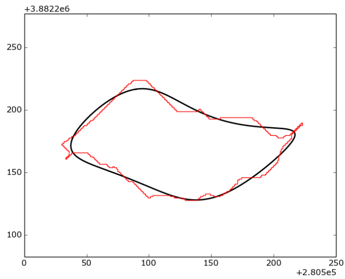
Fig. 3: Example of a non-normalized Fourier ellipse (black) being plotted on top of a shapefile outline (red).
